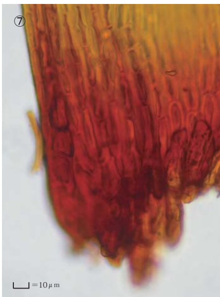
①②③④⑤⑥ Cells at apex of stem leaf. ⑦ Median laminal cells of stem leaf. ⑧ Cells at base of stem leaf.
